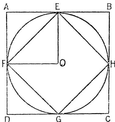
FIG. 7.—RELATION BETWEEN SQUARES AND CIRCLES.
